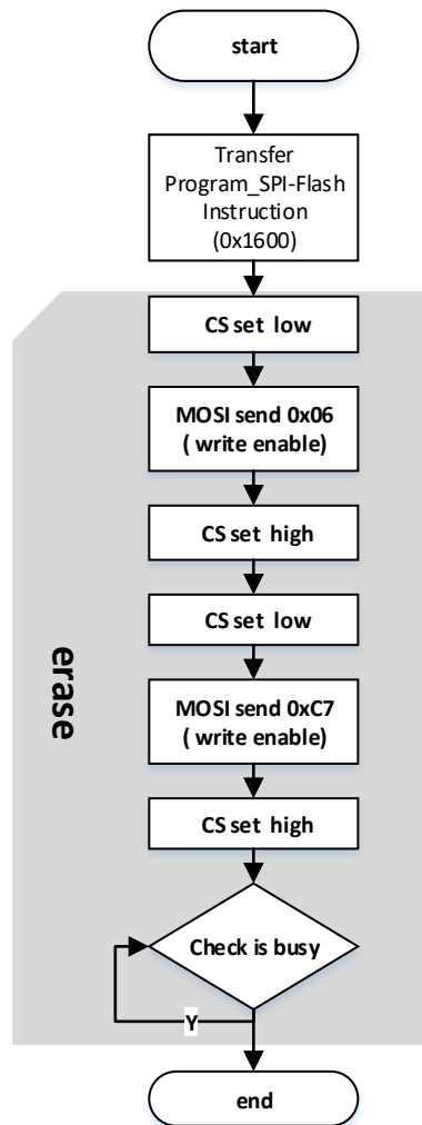
Figure 7-45 The Flow Chart of Erasing SPI Flash
